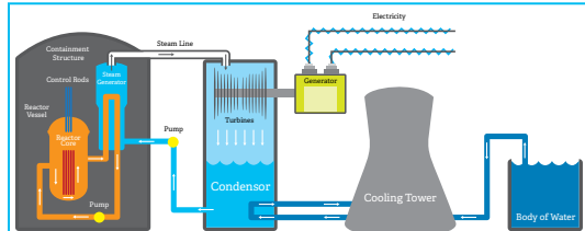
How Plant Vogtle Works
