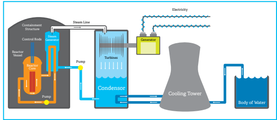
Typical Pressurized Water Reactor (PWR) Design
